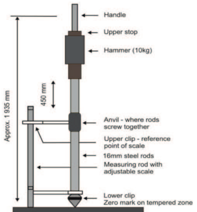
5.8 - Dynamic cone penetrometer
