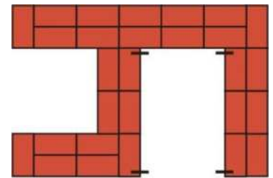
6th Course. Second set if steel lugs fitted
